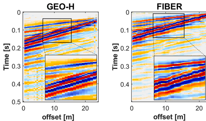
Fig. 6. Example of trace-normalized seismograms from Layout 3: left, horizontal in-line geophones (GEO-H); right, fiber optic sensors (FIBER). It is visible the effect of the 2 m resolution in the fiber optic data.
